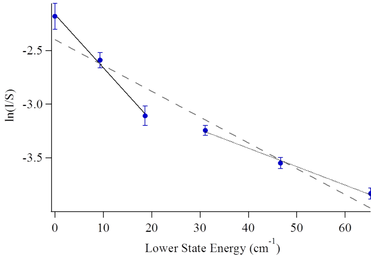
Figure 2.9: A Boltzmann diagram of the rotational distribution of \text{HN}_2^+ shown with 2\sigma error bars. The fit to the low J (R(0), R(2), and R(3), solid line) gives a temperature of \sim 29 K, while the fit to the high J values (R(4)–R(6), dotted line) gives a temperature of \sim 84 K. The dashed line corresponds to a fit to all J values.
