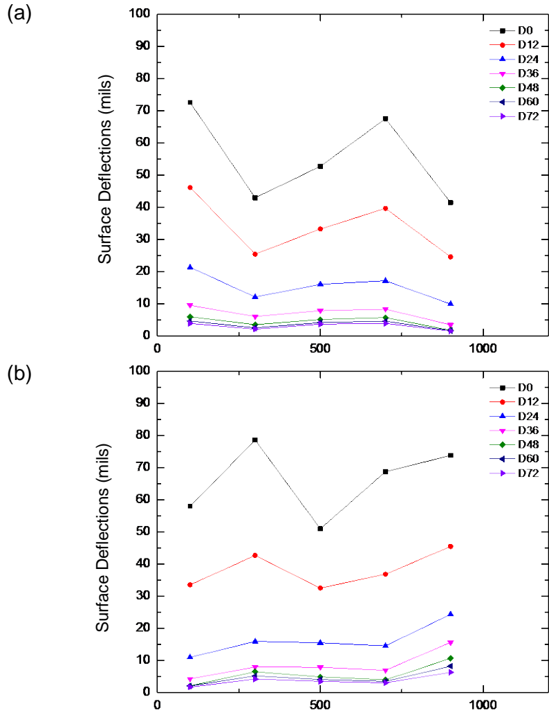
Figure A.6: Deflection basins obtained in south direction from the field during (a) Set 1, and (b) Set 3 FWD testing efforts for pavement section 6.
