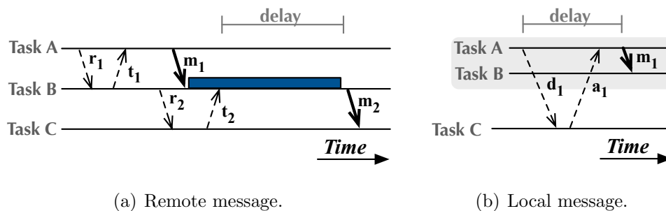
Figure 2.5: Latency overhead scenarios in pessimistic message-logging.
