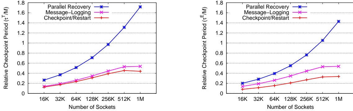
(a) Relative checkpoint period using \tau^T . When execution time is to be minimized, the checkpoint period of checkpoint/restart and message-logging converges to a half the failure rate. Parallel recovery manages to checkpoint much less often, due to its acceleration during recovery.
