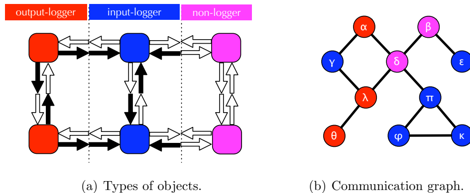
Figure A.3: Different message-logging objects.
