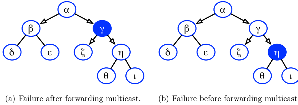
Figure 6.4: Different failure scenarios for a multicast operation.
