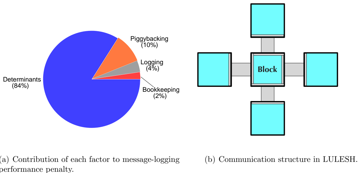
Figure 3.1: Performance cost of determinants in LULESH. The main source of the performance penalty of message-logging with LULESH comes from determinants. The communication structure of LULESH, however, suggests there is a way to avoid all determinants.
