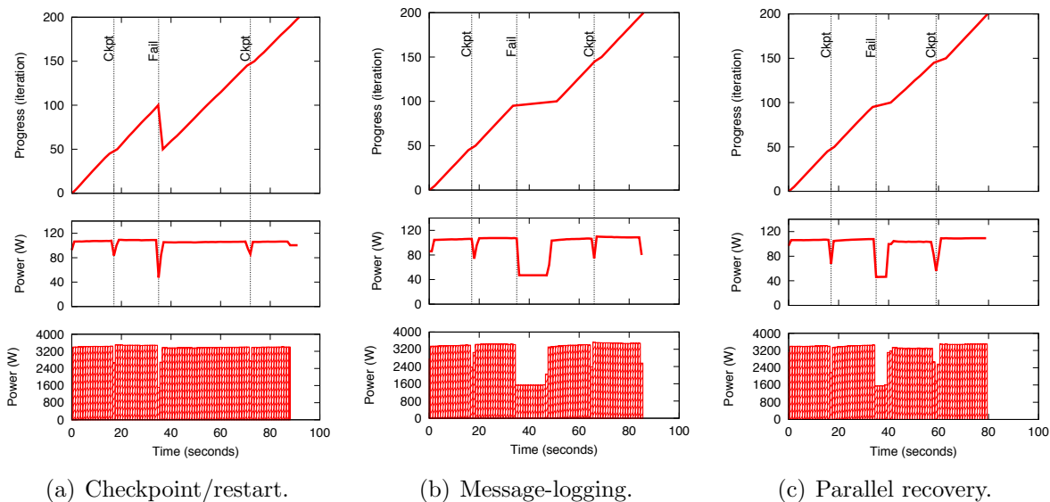
Figure 2.12: Energy profile of different fault-tolerance methods. Message-logging is able to substantially decrease the energy consumed during recovery. In addition, parallel recovery manages to reduce the recovery time to a fraction.
