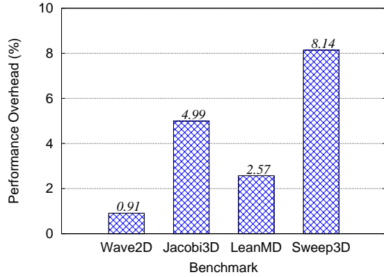
(b) Performance overhead of causal message-logging on different benchmarks.
