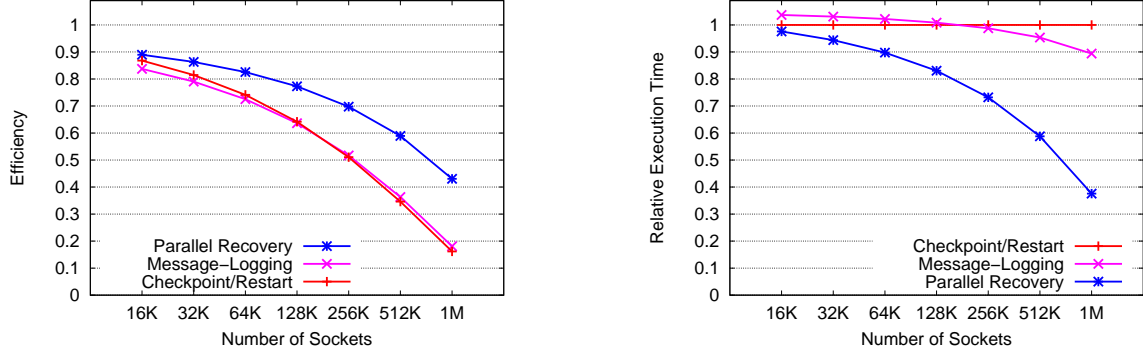
(a) Efficiency of fault-tolerance protocols at large scale. In a machine with more than 256K sockets, parallel recovery improves efficiency for more than 20%.
