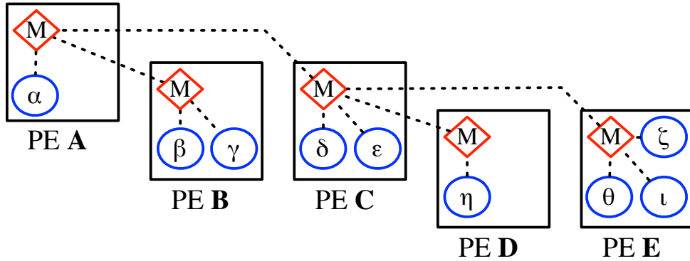
Figure 6.6: Implementation of collective-aware message-logging. Each PE has a special object called a manager that handles the collective communication operations.
