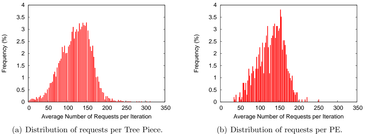
Figure A.2: Distributions of average number of requests per iteration on ChaNGa.
