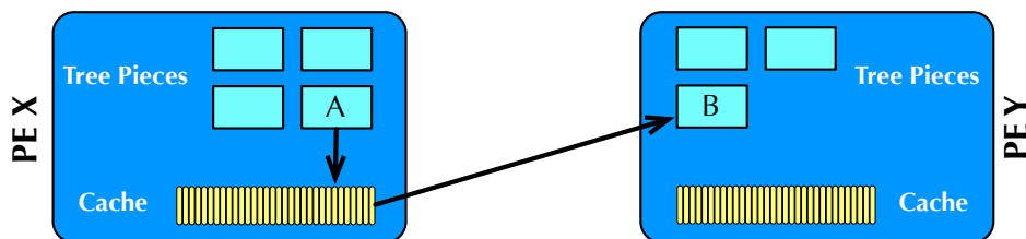
Figure A.1: Simplified diagram of objects in ChaNGa. A Tree Piece that requires the particle information of another Tree Piece will first contact its local Cache to avoid a remote transmission. If the local Cache has the particle message, it will provide them, otherwise it will contact the remote object.
