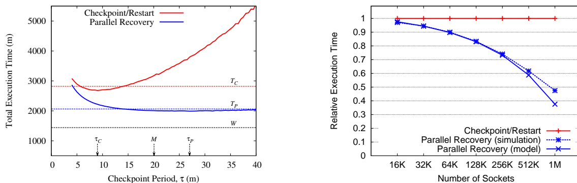
(a) Effect of checkpoint period in total execution time. The minimum of checkpoint/restart is reached at a much smaller value than parallel recovery.
