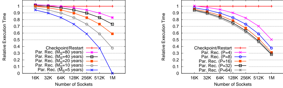
(a) Effect of different values of M_S . The higher the failure rate, the more relative benefits of parallel recovery with respect to checkpoint/restart.
