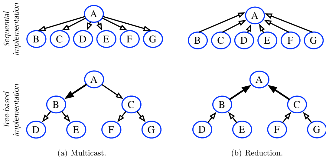
Figure 6.2: Minimizing memory overhead in collective communication operations.
