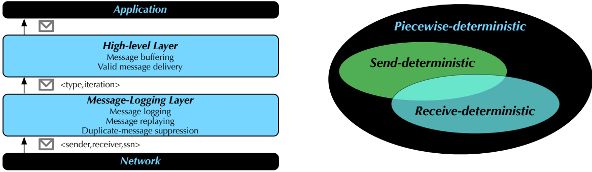
(a) Separation of concerns with the fast message-logging protocol.
