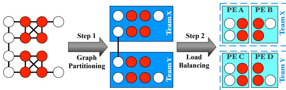
Figure 5.4: Multilevel load-balancing framework for team formation. The first step uses a graph partitioning tool to obtain teams with similar total load but with a small edge cut between them. The second step refines the load distribution among the PEs of each team.
