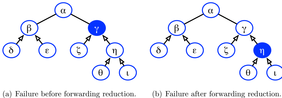
Figure 6.5: Different failure scenarios for a reduction operation.
