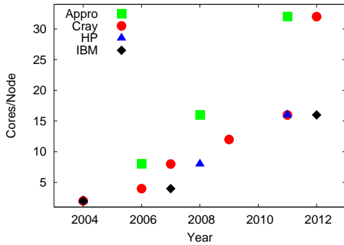
(a) Historical view of number of cores per node in systems from the four major vendors of supercomputers.
