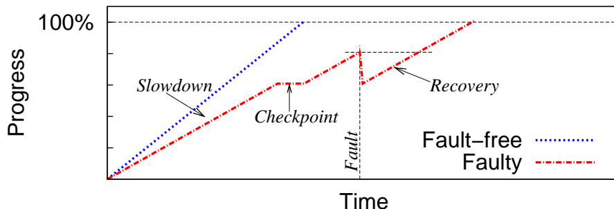
Figure 1.2: Progress diagram. It shows the progress rate as the measure to determine how efficient a fault tolerance solution is.
