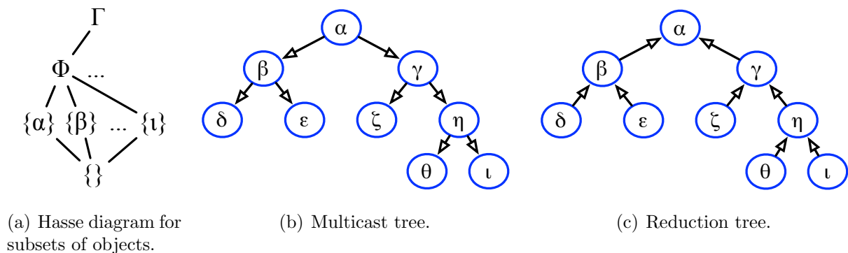
Figure 6.3: Spanning tree for multicast and reduction operations.
