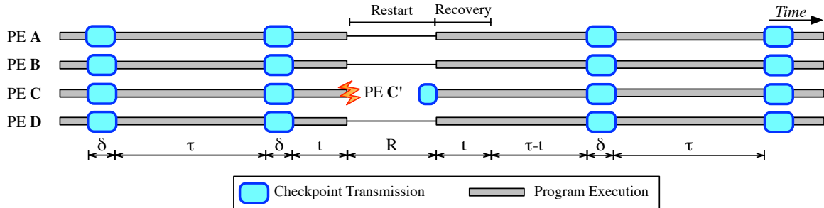
Figure 4.2: Execution model example. The system takes periodic checkpoints and rolls back to the most recent checkpoint in case of a failure.
