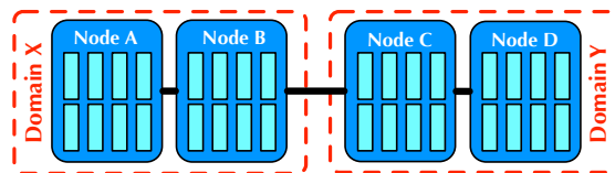
Figure 7.9: Node-failure correlation in multicore-node systems.
