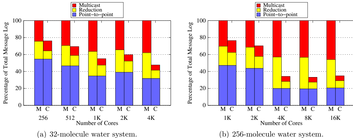
Figure 6.8: Memory overhead reduction in OpenAtom with CAML. The figure contrasts simple causal message-logging (represented by “M”) and the CAML algorithm (represented by “C”)
