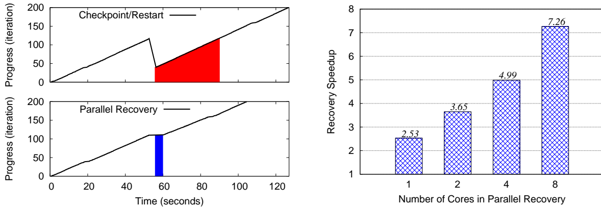
(a) Progress rate in fault-tolerance protocols. Shaded areas represent recovery time. (b) Parallel recovery with causal message-logging. Recovery time can be substantially reduced.
