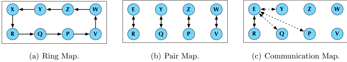
Figure 7.6: Different mappings for storing checkpoints and determinants. If a node fails along with other node having a checkpoint or a determinant, recovery is compromised.
