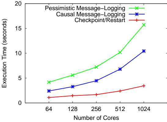
(a) Performance overhead of message-logging protocols in an extreme communication-bound scenario.
