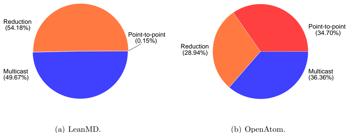
Figure 6.1: Communication volume captured by collective communication operations. LeanMD practically sends all the information through either multicast or reduction operations. OpenAtom uses collectives heavily and two-thirds of the communication load travels through collectives.
