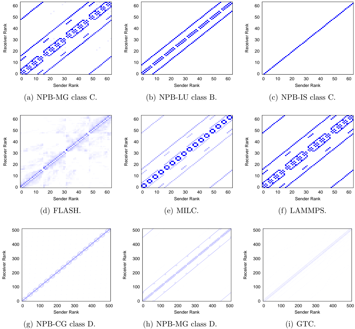
Figure 5.2: Communication graphs of several parallel programs. There is usually a clear clustering structure of the tasks, which causes most of the communication to be enclosed within the clusters.
