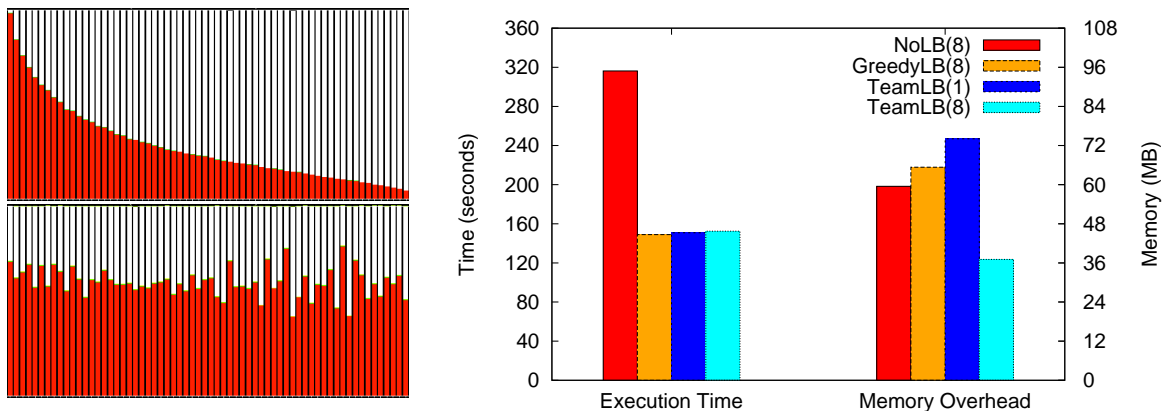
(a) Effect of load balancing in NPB-BT multizone.
