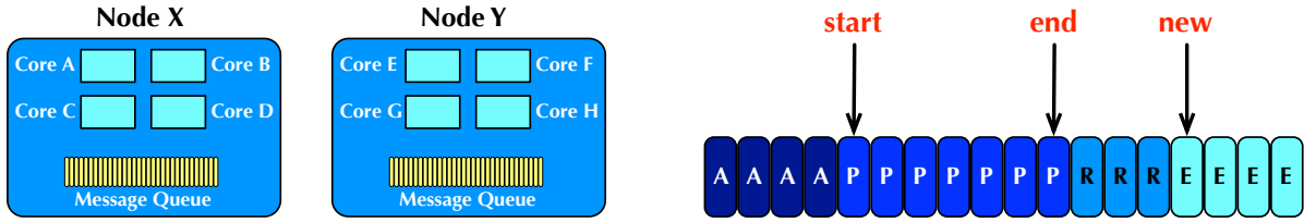
(a) A multicore-node system. Each node contains several cores that shared data structures for communication.
