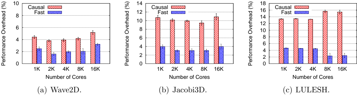
Figure 3.6: Performance overhead of fast message-logging. It approximately reduces performance overhead to a half when compared with causal message-logging.
