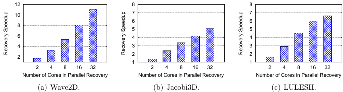
Figure 3.7: Parallel recovery in fast message-logging. The more cores are used to recover, the faster the recovery.
