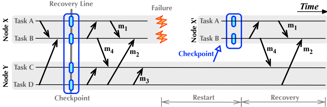
Figure 2.3: Message-Logging with coordinated checkpoint. The same example as in Figure 2.2 is presented, but this time using message-logging. Only tasks in node X are forced to roll back. Messages are re-sent by other nodes and determinants help to ensure reception order is the same as before the crash.
