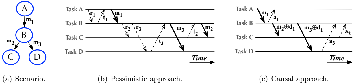
Figure 2.4: Message logging protocols. Using a broadcast spanning tree as a scenario, pessimistic and causal message-logging are contrasted. The causal variant incurs less latency overhead, but it increases bandwidth consumption.
