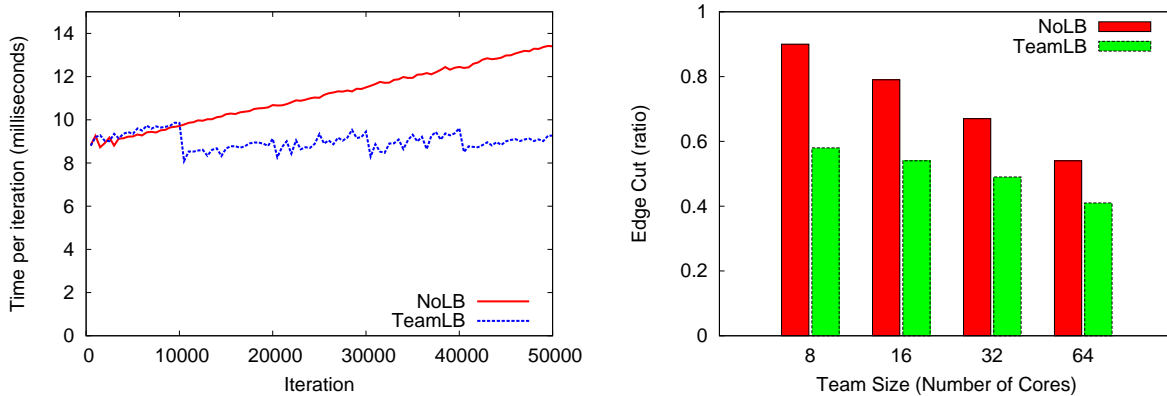
(a) Effect of dynamic load balancing in LBTest. (b) Impact of team size in reducing memory overhead.
