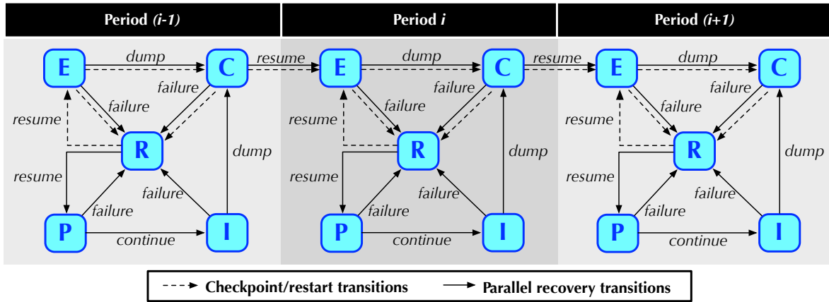
Figure 4.7: Simulation of fault tolerance methods. The state diagram presents the different states in which the application can be during an execution.
