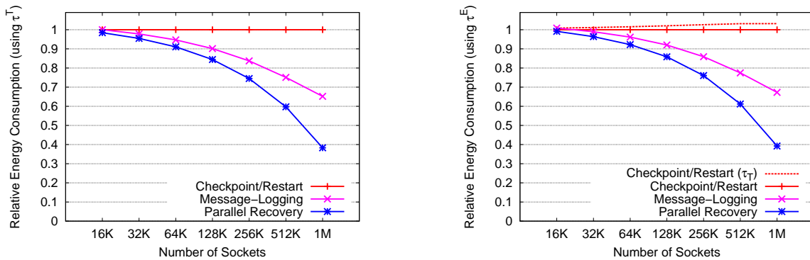
(a) Energy consumption using \tau^T . Both message-logging and parallel recovery perform better than checkpoint/restart all along the range.
