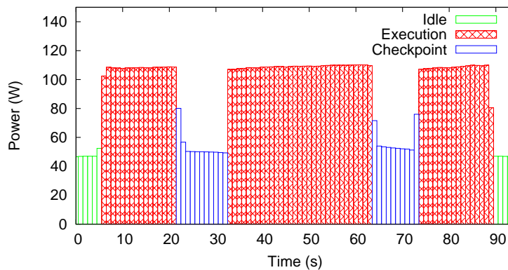
Figure 2.11: Power levels during checkpoint/restart. At checkpoint time, the power draw goes down to almost the idle power level. During execution, the power draw reaches a higher level. The maximum power draw depends on the application and how intensely it uses the computational resources.
