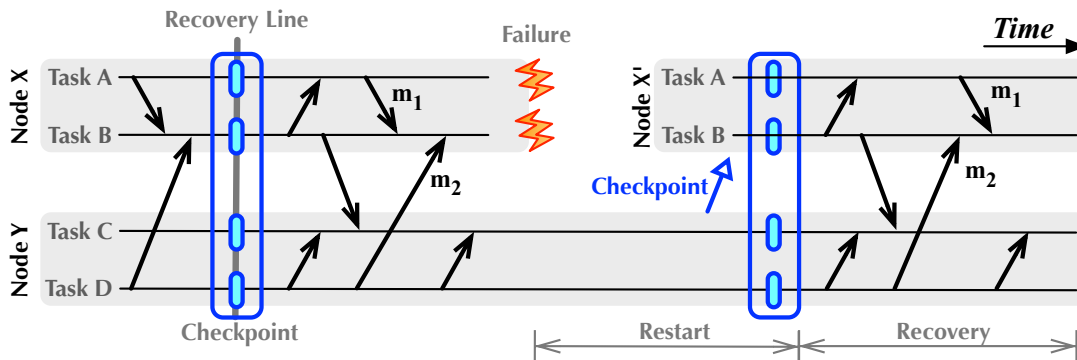
Figure 2.2: Coordinated Checkpoint/Restart. All tasks in the system checkpoint in a coordinated fashion. Often times the programmer triggers the checkpoint at global synchronization points in the application.
