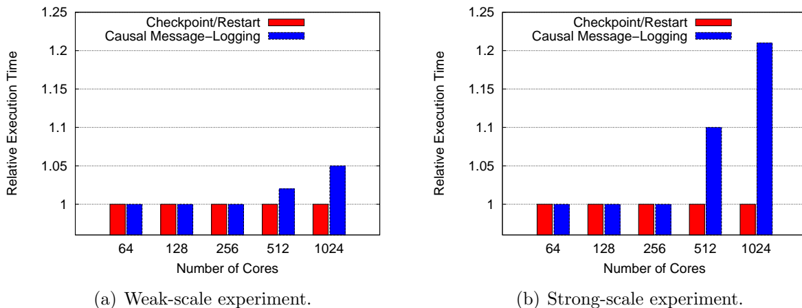
Figure 2.9: Overhead in scaling causal message-logging. The weak scale experiment shows causal message-logging scales well. However, the strong scale experiment suggest the communication overhead starts dominating at the right extreme of the scale.
