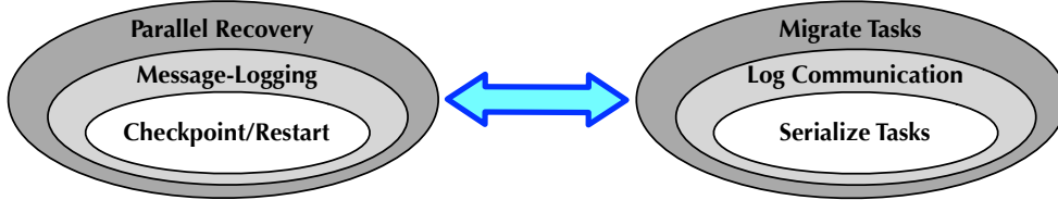
Figure 4.1: Hierarchical organization of protocols. Checkpoint/restart is the base case that allows tasks to be serialized. Message-logging can be seen as an extension to that base case where communication is logged. Furthermore, parallel recovery extends message-logging by allowing tasks to migrate.
