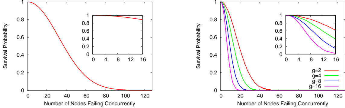
(a) Multiple-node failure survival probability in checkpoint/restart. (b) Multiple-node failure survival probability in message-logging for different g values.
