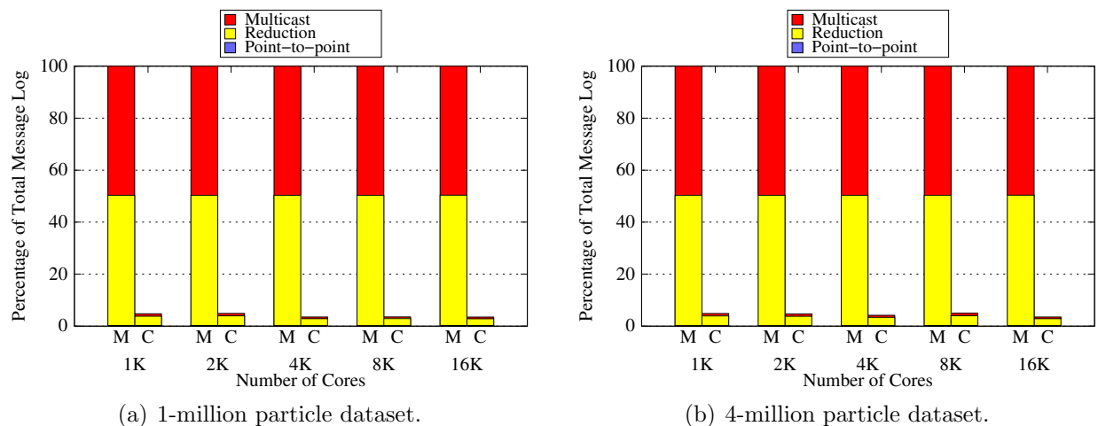
Figure 6.7: Memory overhead reduction in LeanMD with CAML. The figure contrasts simple causal message-logging (represented by “M”) and the CAML algorithm (represented by “C”).
