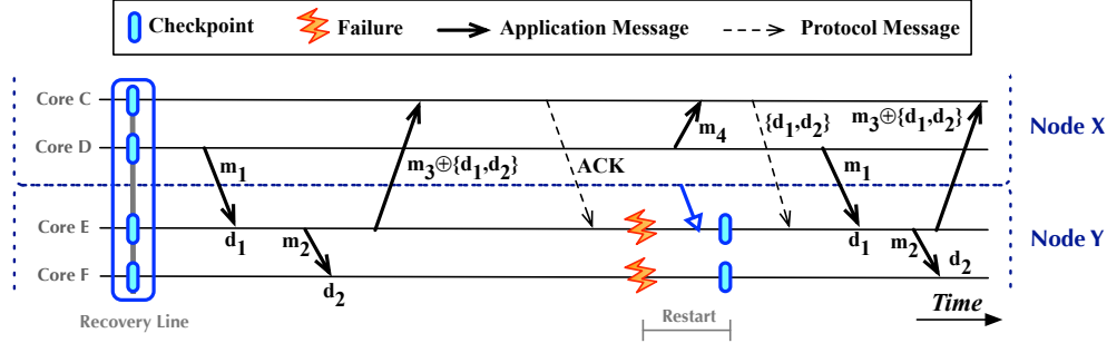
Figure 7.5: Sample execution of an application using the message-logging protocol for multicore-node systems. All message receptions create determinants, but only inter-node messages piggyback determinants.
