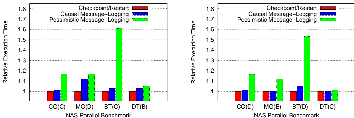
(a) Overhead of message-logging protocols with 256 cores on Abe.
