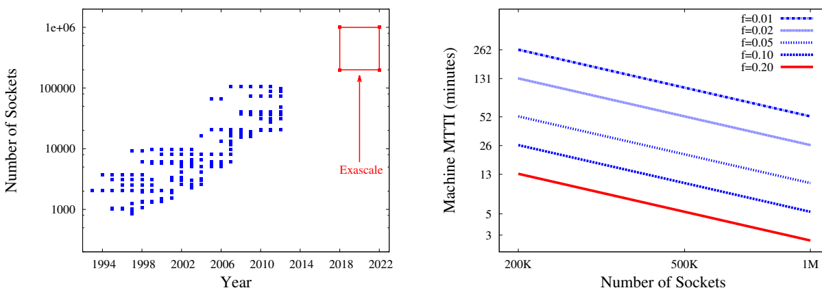
(a) Historical view of the number of sockets in the top 10 largest systems. An exascale machine is expected to have more than 200,000 sockets and to be available between 2018-2022.
