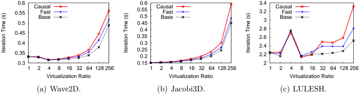
Figure 3.5: Effect of virtualization ratio on performance. Stencil codes admit a high virtualization ratio without sacrificing a significant portion of its performance.
