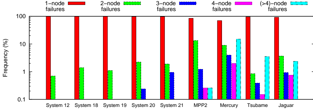
Figure 7.2: Distribution of failures according to the number of nodes affected. For all systems in Table 7.1 the distribution is very skewed: a high percentage of the failures involve only one node.
