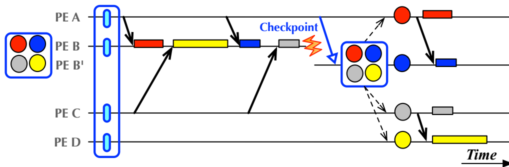
Figure 2.6: Parallel recovery in message-logging.
