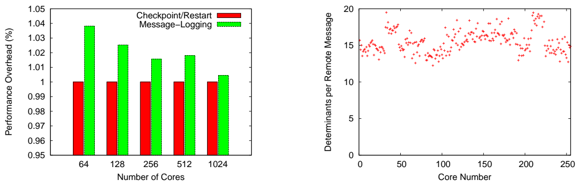
(a) Performance overhead of message-logging with respect to checkpoint/restart. (b) Average number of determinants per remote message.
