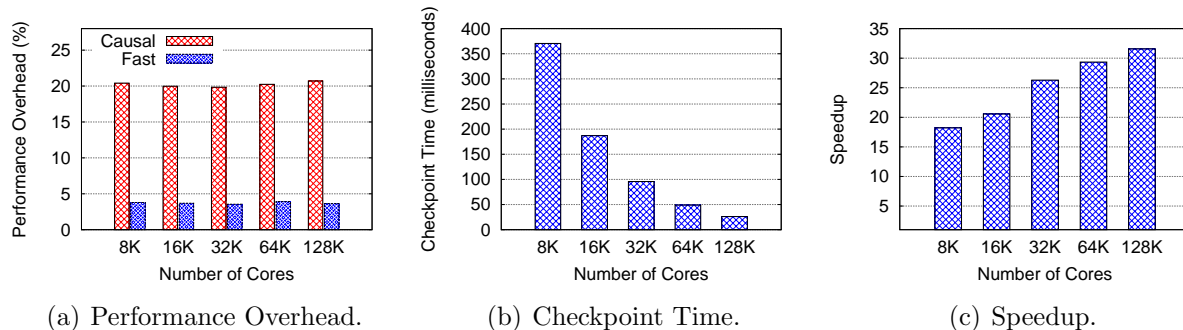
Figure 3.8: Large strong-scale experiment with LULESH. Fast message-logging keeps a low performance overhead, fast checkpoint and fast recovery, compared to checkpoint/restart.
