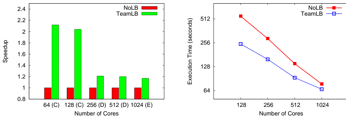
(a) Effect of TeamLB when scaling NPB-BT multizone.
