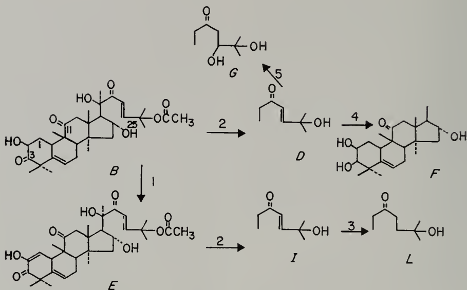
Fig. 3. — Suggested plant evolution of cucurbitacins B, E, D, I, F, G, and L. Numbers refer to specific enzymes involved: 1) cucurbitacin \Delta^1 dehydrogenase, 2) cucurbitacin acetylsterase, 3) cucurbitacin \Delta^{23} reductase, 4) cucurbitacin C3-hydroxylase, and 5) cucurbitacin C24-hydroxylase (Lavie & Glotter 1971).
