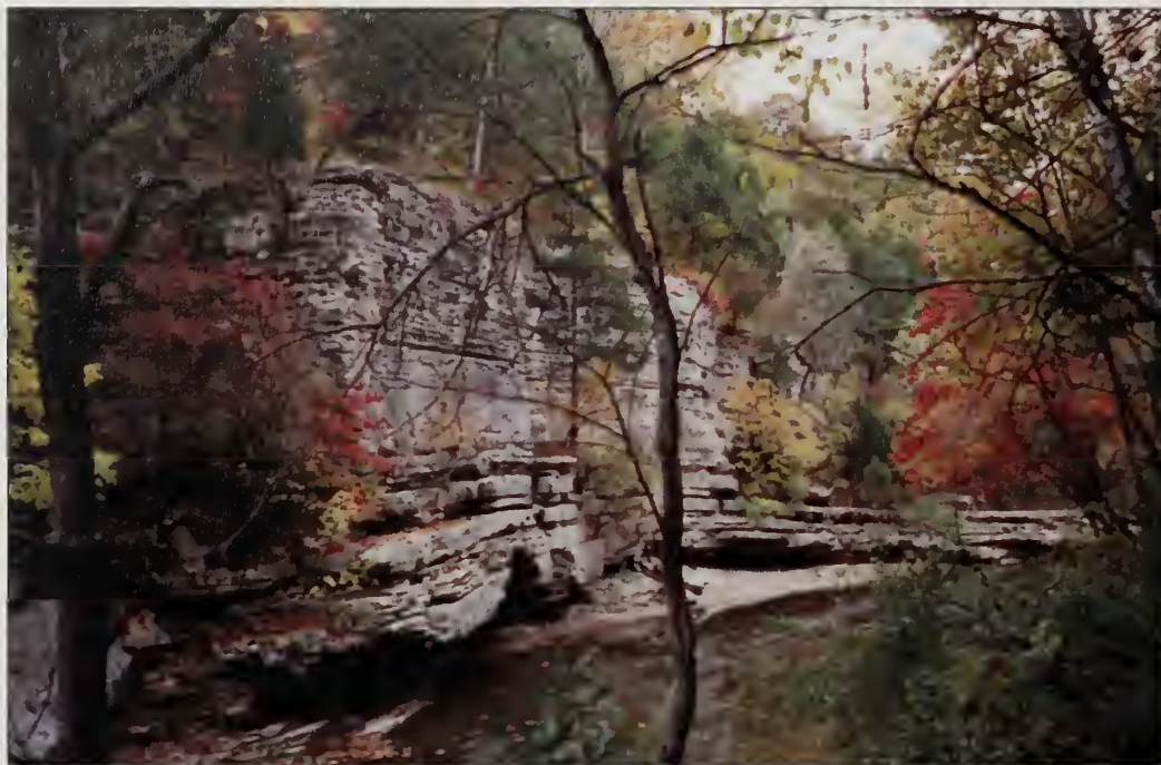
Figure 25 Limestone bluffs of the well-bedded St. Louis Formation bound Fountain Creek and show numerous dissolution features. (Photograph by Samuel V. Panno.)
