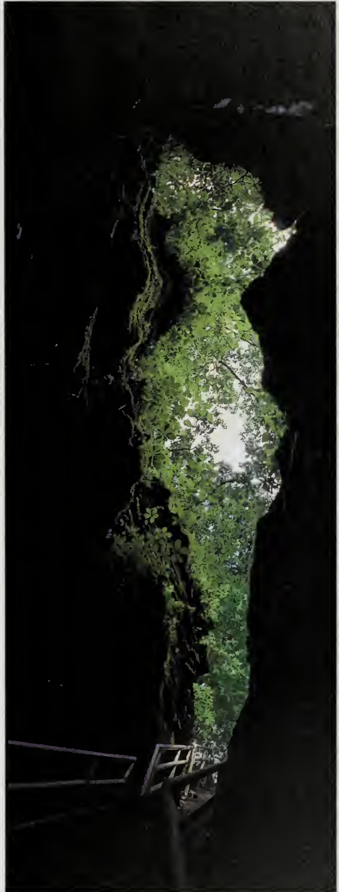
Figure 8 The entrance to Illinois Caverns, as viewed from the cave floor, is an east-west-trending solution-enlarged crevice at the bottom of a sinkhole (Panno et al. 2004a).
