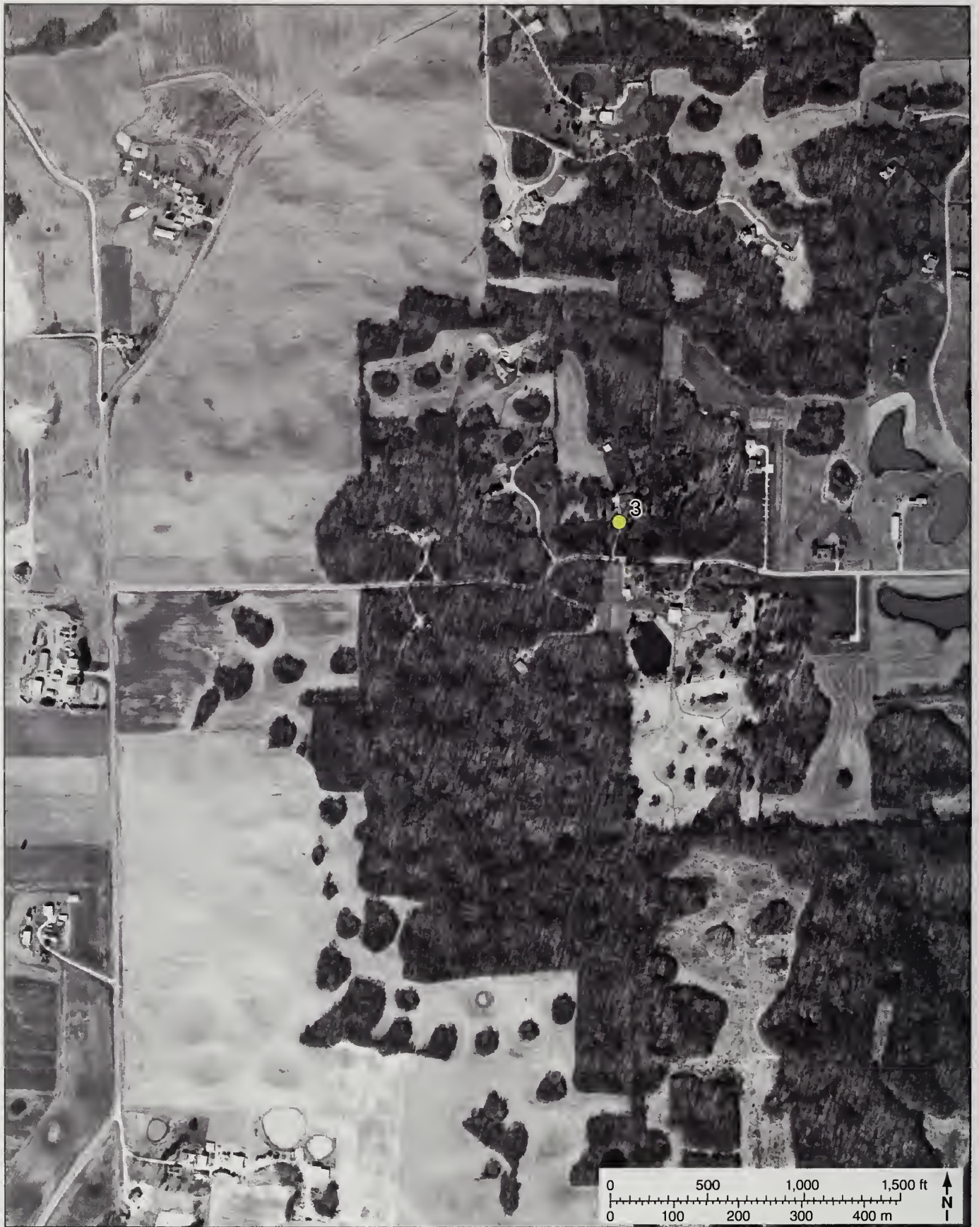
Figure A5 USGS NAPP aerial photograph of the Stemler Cave Woods Nature Preserve area and associated karst terrain acquired on March 3, 2005.
