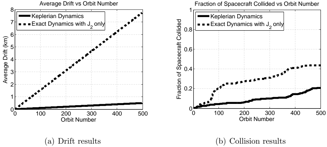
Figure 7: Simulation results of a linearized concentric PRO swarm with no crosstrack drift
