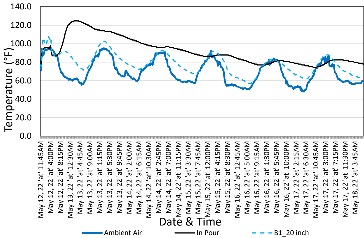
Figure 16. Graph. Temperature variation with time of specimens for the May 12, 2022, cast.
