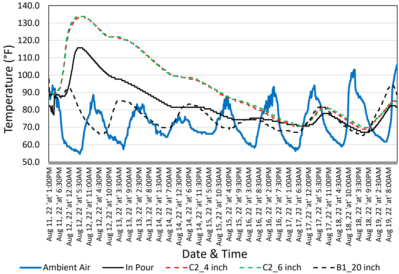
Figure 23. Graph. Temperature variation with time of specimens for the cast on August 11, 2022.
