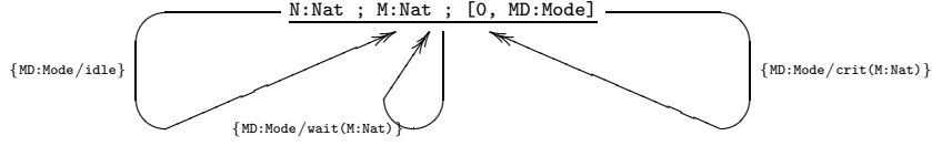
Fig. 2. Finite transition system \text{Reach}_{\mathcal{N}_{\mathcal{R}}}^{\leq_E}(\mathbb{N}:\text{Nat} ; \mathbb{M}:\text{Nat} ; [0, \text{MD}:\text{Mode}])
