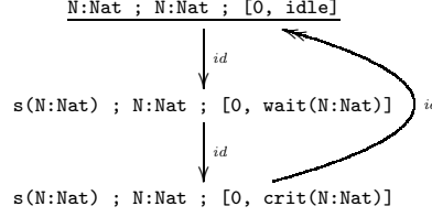
Fig. 3. Finite transition system \mathcal{R}eac\hbar_{\mathcal{N}\mathcal{R}}^{\leq_E}(\mathbf{N:Nat} ; \mathbf{N:Nat} ; [0, \mathbf{idle}])
