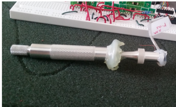
Figure 4.10: Probe tip connected to a uniform cylindrical syringe of 7.5 [mm] diameter. A jump discontinuity between the probe tip and the syringe was created using a washer as a flat plane, fused to the probe tip using a glue gun. To measure the two-port parameters of the probe tip, the plunger depth was varied (and carefully measured) to create test cavities of known impedance.
