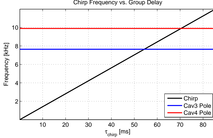
Figure 4.5: Chirp frequency as a function of group delay. The approximate pole frequencies are marked in red and blue for cavities 3 (about 18 [mm] long) and 4 (about 22 [mm] long).
