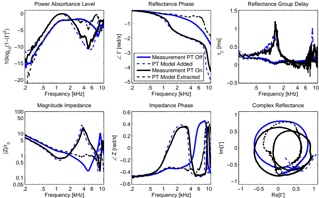
Figure 4.11: Measurements of the Mimosa Acoustics average-ear simulator with (solid black) and without (solid blue) the probe tip. By adding or extracting (subtracting) the computational model for the probe tip (Fig. 4.6), each measurement is used to predict the other (dashed lines). The estimate is better when adding the probe tip on (dashed blue), rather than extracting its effects (dashed black).
