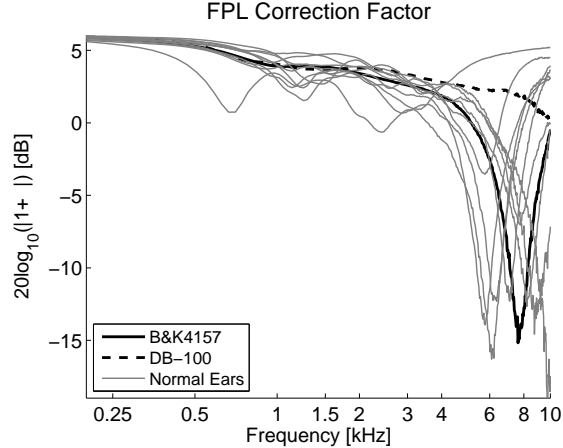
Figure 2.6: Forward pressure level normalization factor |1 + \Gamma| , which corrects for the ear-canal standing wave, for 10 normal ears and two ear simulators from Voss & Allen (1994). At the frequency of the null, the phase of the complex reflectance is approximately 180 degrees (Withnell et al., 2009). The frequency of the null critically depends on the round-trip delay between the probe tip and the TM (Eq. 2.28d). This delay is different for each ear, as it depends on the insertion depth of the probe and the geometry of the ear canal and TM. As the ear-canal delay decreases, the standing-wave null shifts upward in frequency.
