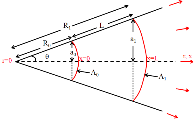
Figure A.8: Example of a conical horn of length L , beginning at x = r - R_0 = 0 . The planar radii at the ends of the horn are specified by a_0 and a_1 . The areas of the iso-pressure curves are given by the spherically convex areas A_0 and A_1 .
