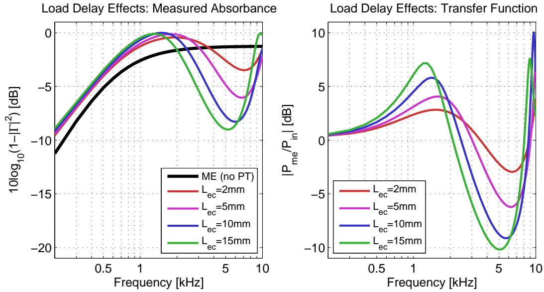
Figure 4.8: Effects of varying load (ear-canal) delay on the measured absorbance at the point of Thévenin calibration (left), and the transfer function across the probe tip and ear canal, from the calibration point to the middle ear (right). Longer ear-canal models (with more delay) produce more extreme changes (from the black curve) due to the variable-area tip. Based on these simulations we conclude that these changes are due to the combination of the jump discontinuity and the delays of the probe tip and ear canal.
