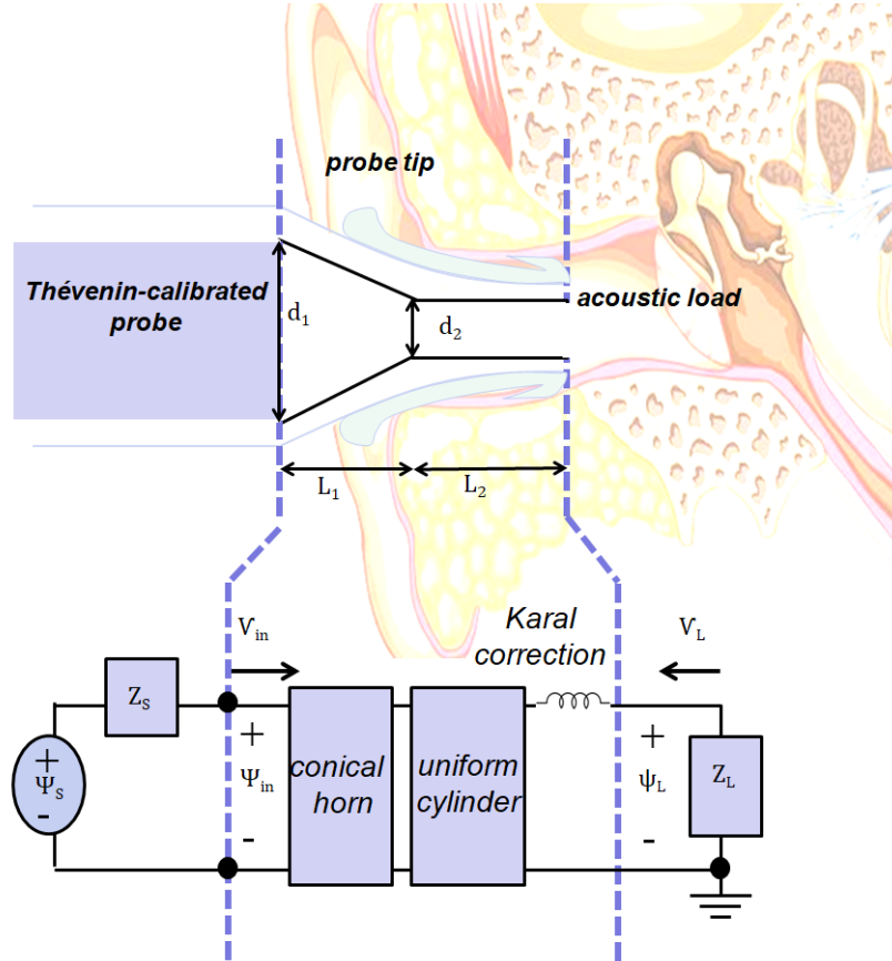
Figure 4.6: Configuration and model for a middle-ear WAI measurement made using the probe tip. The original probe tip studied had d_1 = 7.5 [mm], d_2 = 4.0 [mm], L_1 = 6.5 [mm], and L_2 = 13.3 [mm]. This tip is somewhat large for adult ears.
