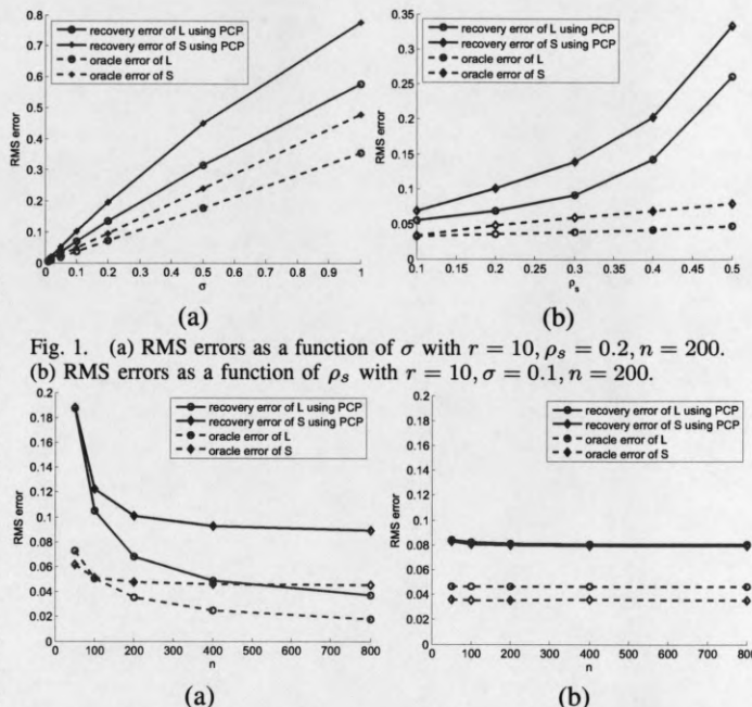
Fig. 2. RMS errors as a function of n with (a) \sigma = 0.1 , \rho_s = 0.2 , r = 10 fixed, (b) \sigma = 0.1 , \rho_s = 0.1 and r = 0.1 \times n growing in proportion to n .
